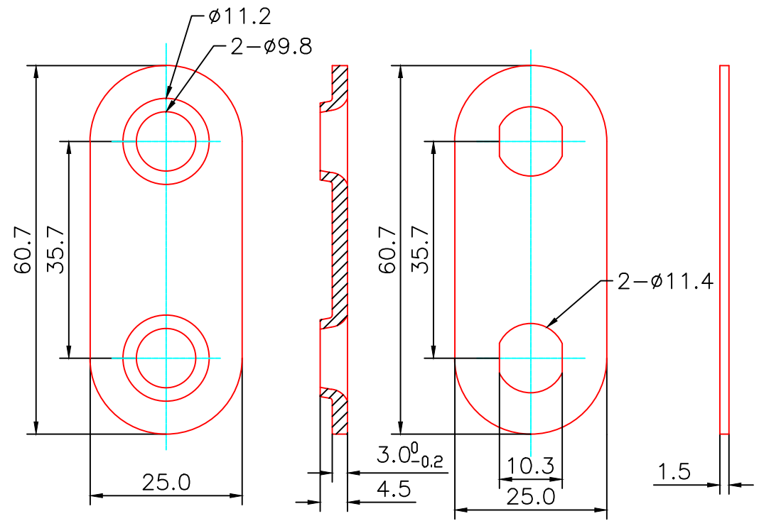
WELDED PLATE
